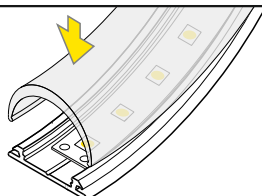
difuzor D klip / D click cover
