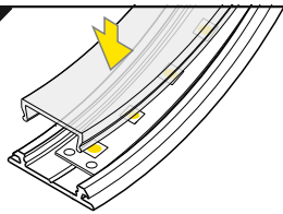
difuzor C klip / C click cover
